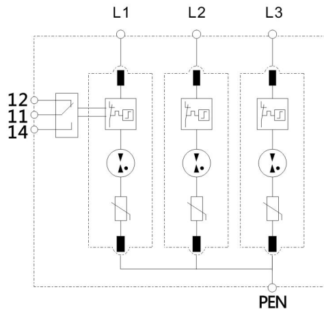
Electrical principle
